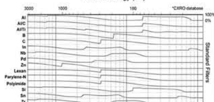
XUV ultra-thin filter
