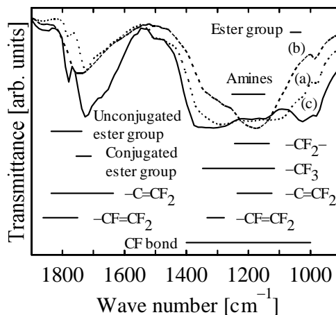
Fig. 1. FTIR spectra of the films formed with different source materials; (a) sample A, \text{C}_7\text{F}_{16} ; (b) sample B, (\text{C}_3\text{F}_7)_3\text{N}/(\text{C}_4\text{F}_9)_3\text{N} ; and (c) sample C, \text{C}_8\text{F}_{18}/\text{C}_8\text{F}_{16}\text{O} .
