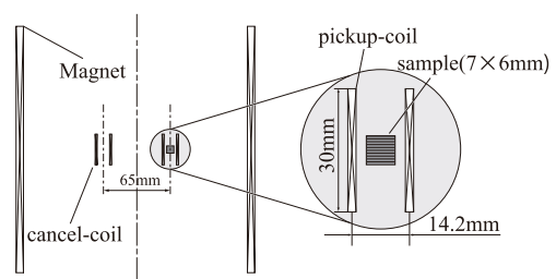
Fig. 2 Measuring system.
