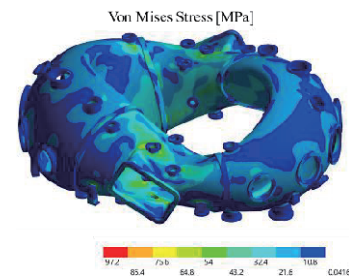
Fig. 9 Results of case 3, stress [MPa].
