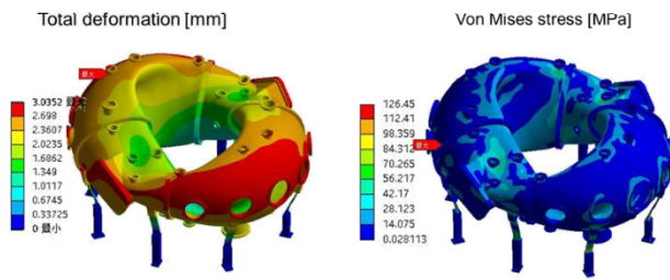
Fig. 8 Results of case 2 (a) deformation [mm], (b) stress [MPa].
