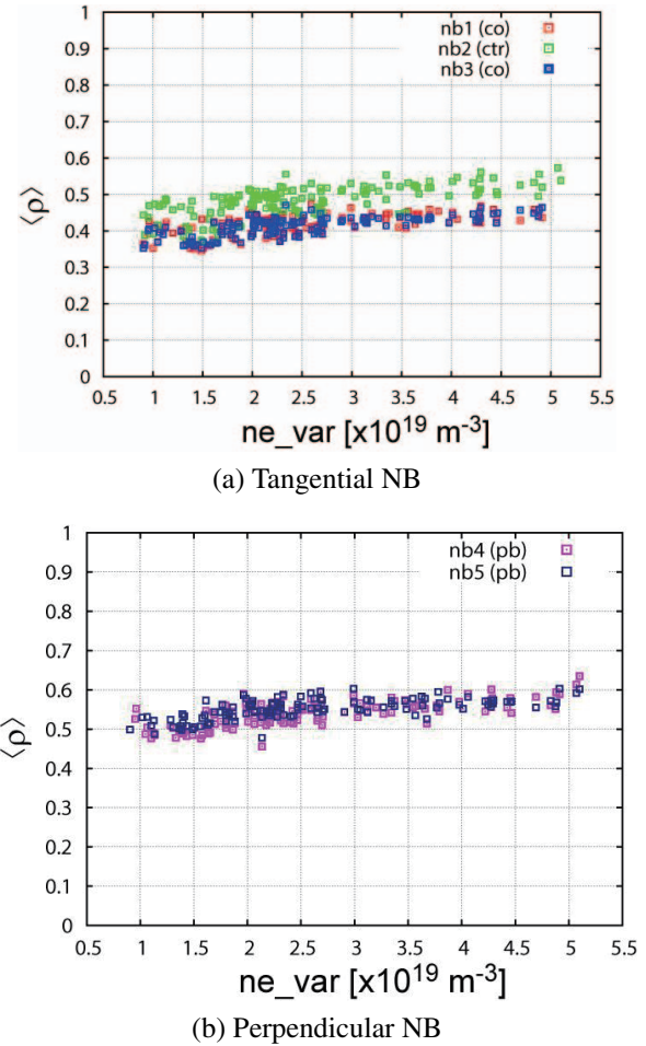
Fig. 6 Effective normalized minor radius for neutron emission rate in the case of (a) tangential NB and (b) perpendicular NB.
