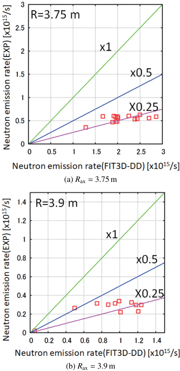
Fig. 5 Comparison of the neutron emission rate between FIT3D-DD results and neutron flux monitor measurements in the case of the low confinement of the fast-ion.
