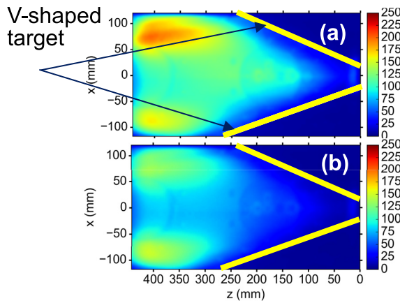
Fig. 6 2D images of visible emission during (a) Kr 100 mbar, (b) Kr 400 mbar injection (without filter, 350 - 380 ms).
