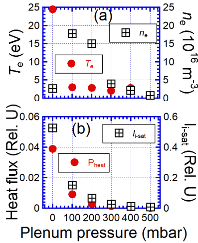
Fig. 5 Dependence of (a) electron density and temperature (measured by probe#1), (b) heat and ion fluxes (corner probe and CM) as a function of the Kr plenum pressure.
