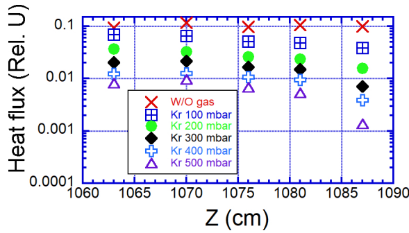
Fig. 3 Dependence of heat flux along the target plate.
