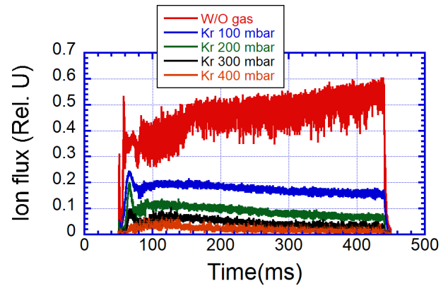
Fig. 4 Time behavior of ion flux measured by the corner probe.
