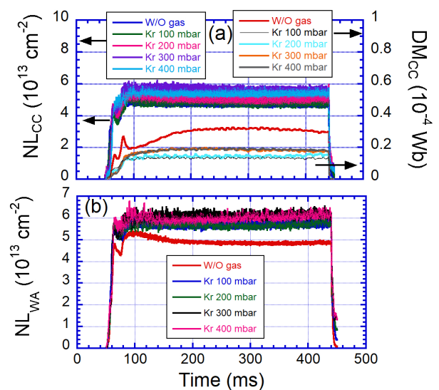
Fig. 2 Time behavior of the (a) electron line density and diamagnetism at the central-cell, (b) electron line density at the west anchor-cell.
