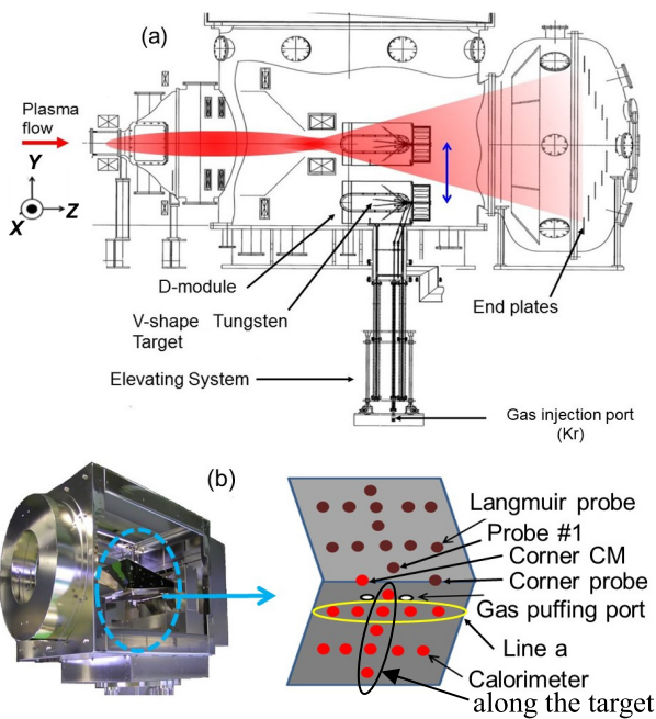
Fig. 1 Schematic view of the (a) GAMMA 10/PDX west plug/barrier-cell to end-cell, (b) D-module.
