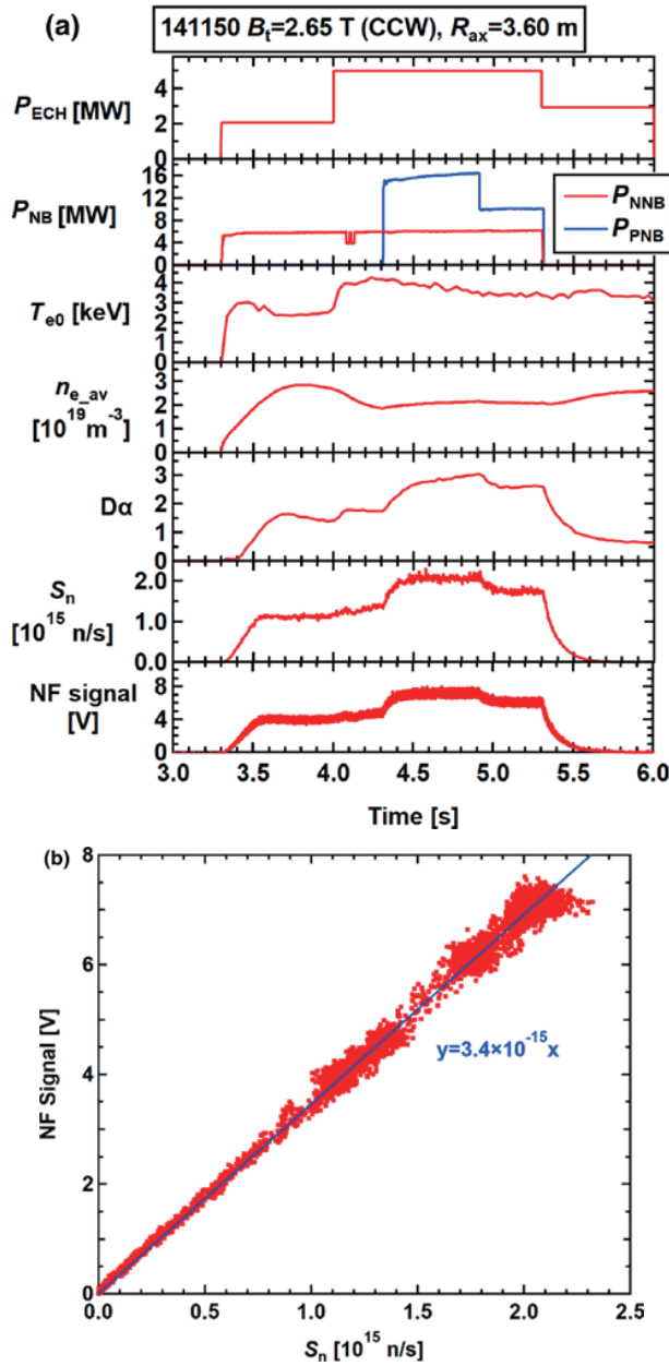
Fig. 3 (a) Time evolution of injection powers of ECH and NBI, T_{e0} , n_{e\_av} , D\alpha , S_n , and NF signal on the MHD quiet discharge. (b) Relation between S_n and NF signal. NF signal linearly increases with S_n .
