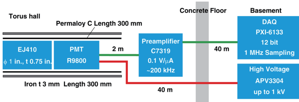
Fig. 1 Block diagram for fast-neutron scintillation diagnostics.
