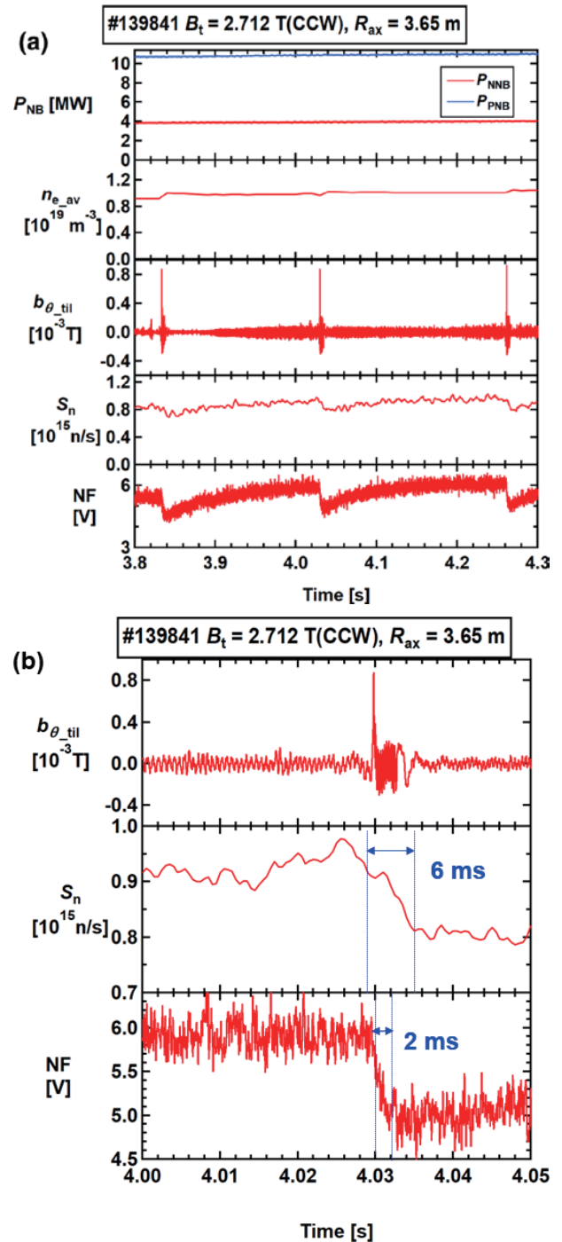
Fig. 4 (a) Time evolutions injection powers of NBIs, n_{e\_av} , magnetic fluctuation amplitude, S_n and NF signal on the discharge with strong MHD bursts. (b) Enlarged figure of (a) Rapid changes of NF signal due to intermittent MHD bursts are observed.
