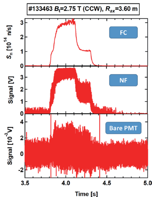
Fig. 2 Time evolutions of S_n , NF signal, and bare PMT signal. The signal caused in PMT by neutron/gamma-ray is three orders smaller than that of the scintillation signal.
