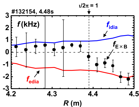
Fig. 2 Radial profiles of the \mathbf{E} \times \mathbf{B} rotational frequency (closed circles), the ion diamagnetic rotational frequency (blue), and the electron diamagnetic rotational frequency (red) in the H-rich plasma as shown in Figs. 1 (a) - (g). The vertical dashed line indicates the \iota/2\pi = 1 resonant surface.
