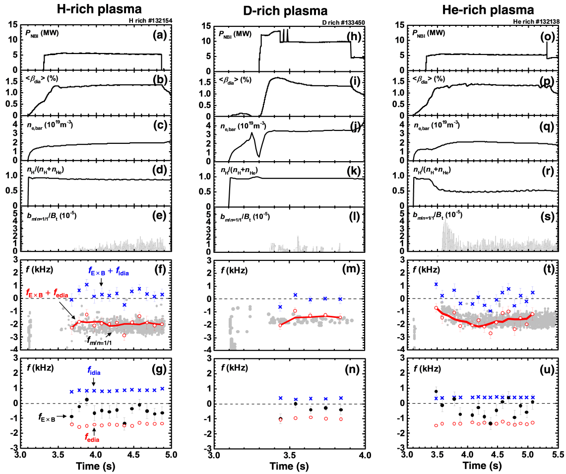
Fig. 1 Time evolution of (a) tangential NBI power; (b) volume-averaged beta value; (c) line-averaged electron density; (d) density ratio of H to He; (e) amplitude of the m/n = 1/1 mode; (f) frequency of the m/n = 1/1 mode, f_{m/n=1/1} (closed circles), \mathbf{E} \times \mathbf{B} rotational frequency adding to ion diamagnetic frequency, f_{\mathbf{E} \times \mathbf{B}} + f_{\text{idia}} (crosses), adding to electron diamagnetic frequency, f_{\mathbf{E} \times \mathbf{B}} + f_{\text{edia}} (open circles), and moving-averaged f_{\mathbf{E} \times \mathbf{B}} + f_{\text{edia}} (line); and (g) \mathbf{E} \times \mathbf{B} rotational frequency (closed circles), ion diamagnetic rotational frequency (crosses), and electron diamagnetic rotational frequency (open circles) in the H-rich plasma. (h) - (n) Same parameters as (a) - (g) in the D-rich plasma. (o) - (u) Same parameters as (a) - (g) in the He-rich plasma. The positive (negative) sign corresponds to the ion (electron) diamagnetic direction in (f), (g), (m), (n), (t), and (u).
