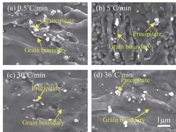
Fig. 6 Microstructure (SEM images) of 12Cr-ODS at 1050 °C for 3 h with different cooling rates, (a) 0.5 °C/min, (b) 5 °C/min (HIP condition), (c) 30 °C/min, (d) 36 °C/min.
