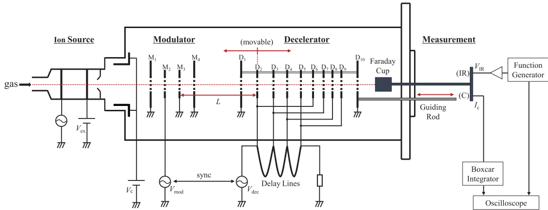
Fig. 1 Schematic view of the experimental device.
