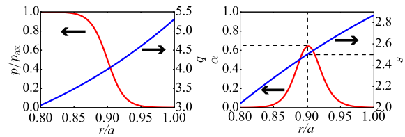
Fig. 1 The shifted circular equilibrium for CBM/RBM instability analysis: the radial profiles of p/p_{ax} and q (left) and the radial profiles of s and \alpha (right), where the beta value at the magnetic axis is p_{ax}/(B_{ax}^2/2\mu_0) = 5 \times 10^{-4} .
