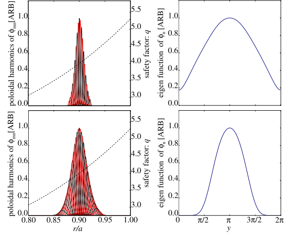
Fig. 3 Radial structure of poloidal harmonics (left) and eigen function in parallel direction (right) of n = 40 mode of \tilde{\phi} in the collisionless limit \eta = 1.0 \times 10^{-10} with d_e^* = d_e (upper row) and d_e^* = 10d_e (lower row).
