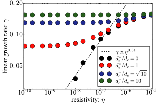
Fig. 2 Linear growth rates of n = 40 CBM/RBM as functions of resistivity for 4 different d_e^* = 0, d_e, \sqrt{10}d_e, 10d_e which correspond to the computational electron masses m_e^* = 0, m_e, 10m_e, 100m_e respectively for d_e^* \propto \sqrt{m_e^*} .
