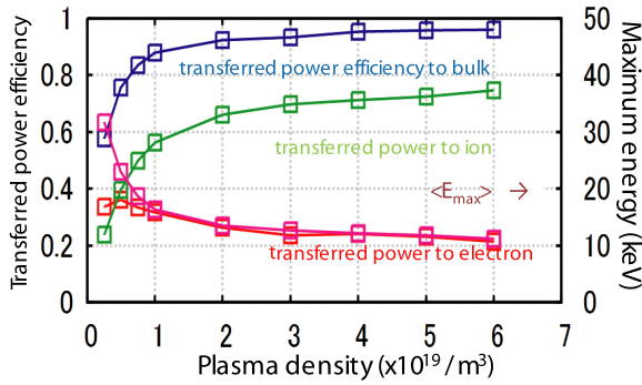
Fig. 3 Density dependence of transferred power efficiency with T_e = 1 keV. In this figure, the blue line shows transferred power efficiency to bulk plasma (ions and electrons). The green and red lines are the efficiency to ion and to electron, respectively. In addition, the purple line shows the maximum energy of ICRF fast ions. The maximum energy shown in the figure is the average value of the maximum energy of each fast ion.
