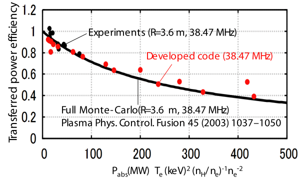
Fig. 2 Efficiencies of developed code and full analyses of part b).
