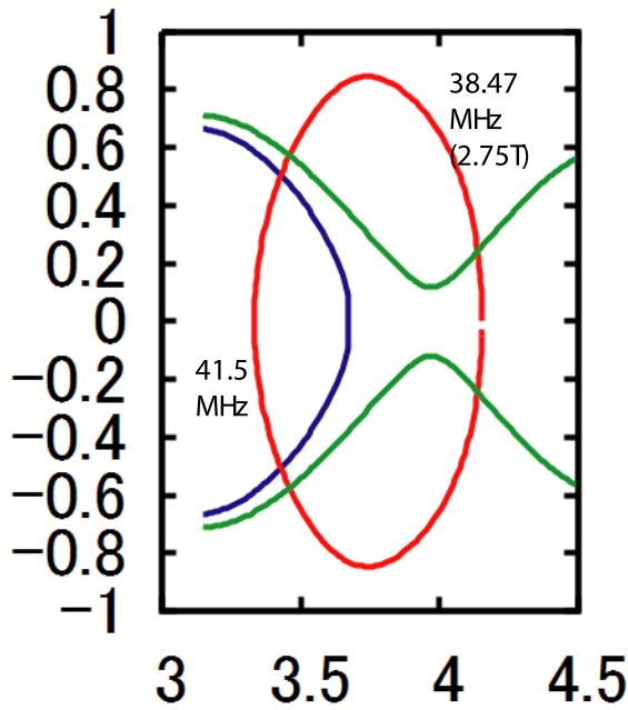
Fig. 8 Resonance layers of 38.47 MHz (green) and 41.5 MHz (blue) on the vertical elongated poloidal plane.
