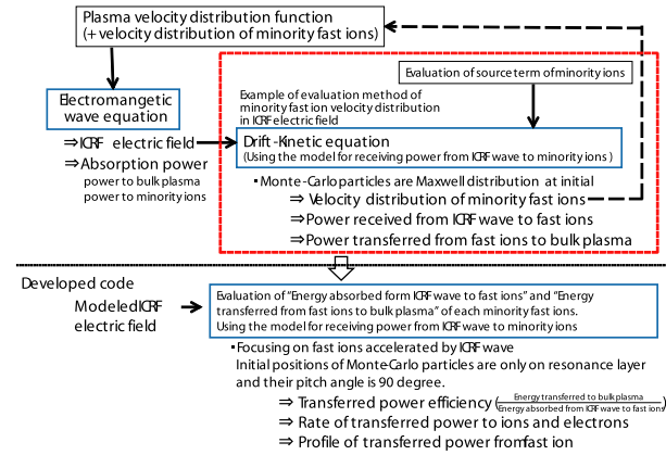
Fig. 1 Overview of models used in developed code and full analysis model of ICRF minority ion heating.
