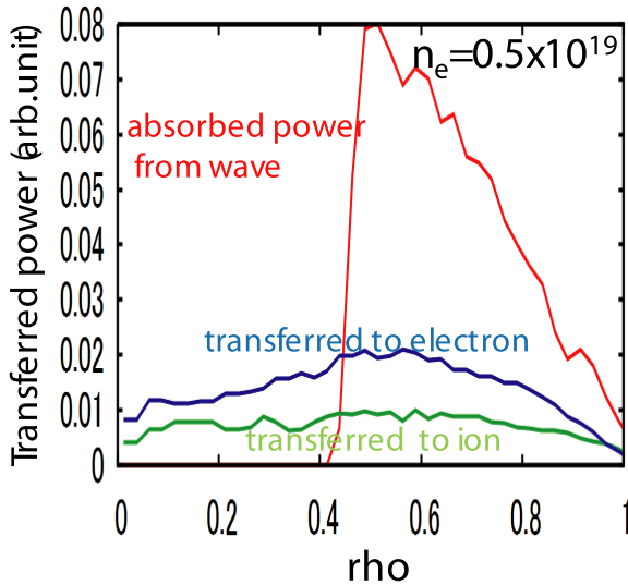
Fig. 4 Typical profiles of the transferred power and absorbed power from wave in the case of T_e = 1 keV and n_e = 0.5 \times 10^{19} \text{ m}^{-3} .
