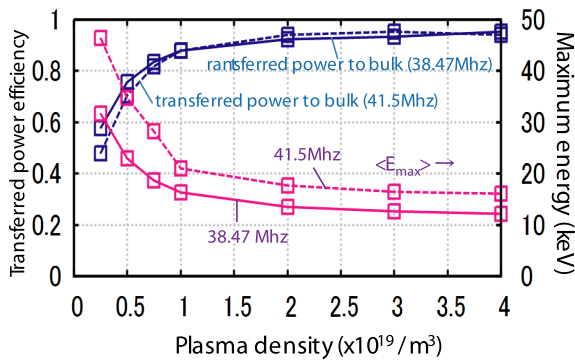
Fig. 9 Difference of transferred power efficiency and maximum energy due to position of resonance layer with T_e = 1 keV.
