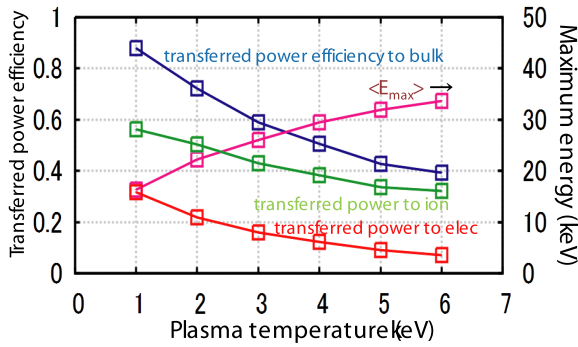
Fig. 6 Temperature dependence of transferred power efficiency with n_e = 1.0 \times 10^{19} \text{ m}^{-3} .
