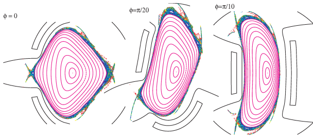
Fig. 7 Relationship between magnetic surfaces, vacuum vessel, and helical coils under geodesic winding on a greatly elongated winding frame ( \kappa = 1.8 ).
