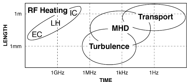
Fig. 1 The range of time and spatial scales of the phenomena in fusion plasmas.
