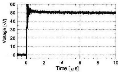
Fig. 5 Waveform of output voltage in case of open circuit load.
