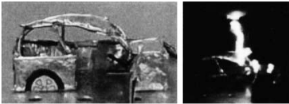
Fig. 9 Long-gap discharge to a simulated vehicle.
