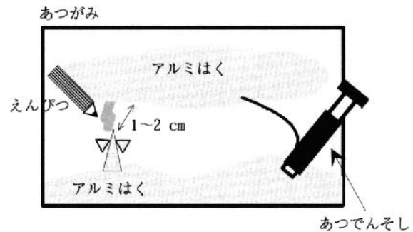
Fig. 16 Schematics of mini-lightning panel.
