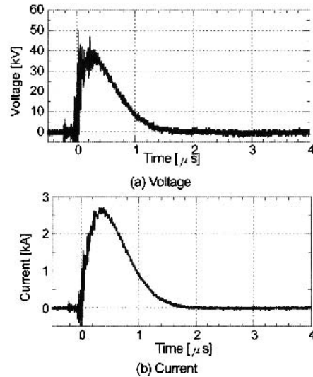
Fig. 6 Waveforms of voltage and current in case of water resistor load with resistance of 12 \Omega .
