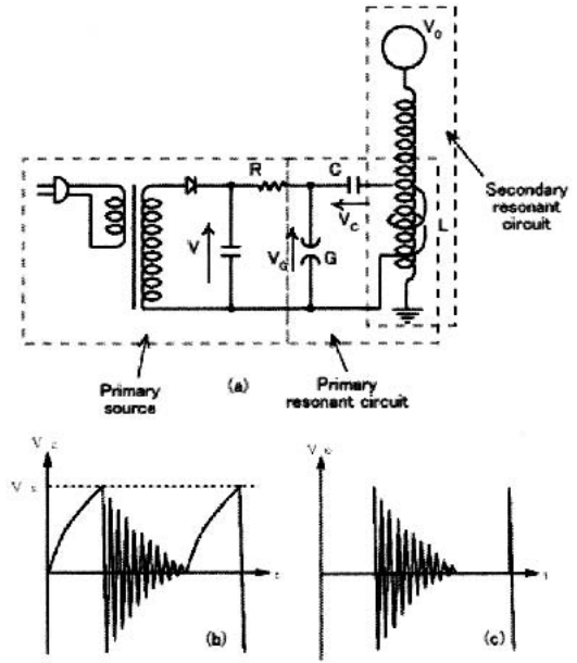
Fig. 10 Electrical circuit of Tesla coil.
