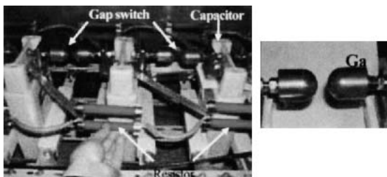
Fig. 2 Photograph of setup of capacitors, gap switches and resistors.
