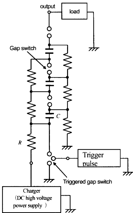
Fig. 1 Equivalent circuit of Marx generator.
