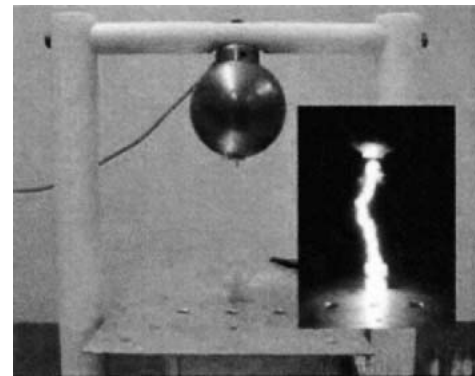
Fig. 7 Long-gap discharge to a human-shaped sponge doll.
