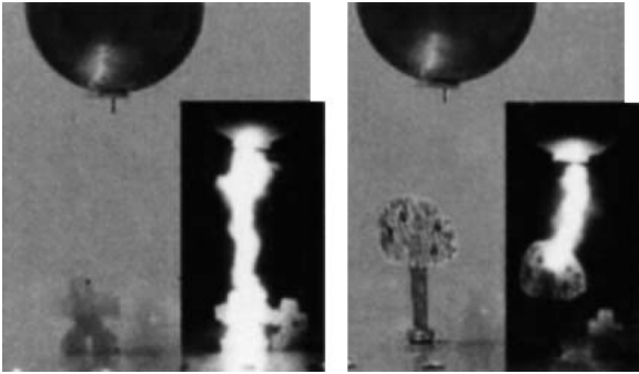
Fig. 8 Long-gap discharge to a higher sponge doll (left photograph) and a simulated tree (right photograph).
