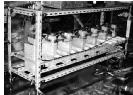
Fig. 4 Photograph of Marx generator.
