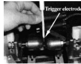
Fig. 3 Photograph of triggered spark gap switch.
