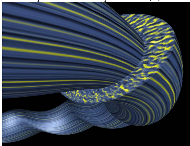
Fig. 1. Turbulent fluctuation in the LHD plasma.
