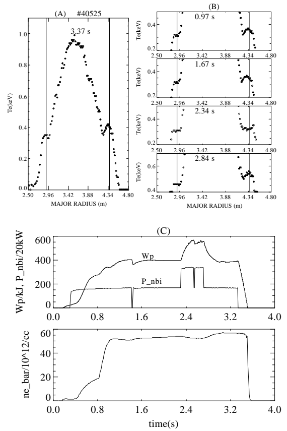
Fig.1. (A) T_e profile with bulges around \iota=1 (vertical lines). (B) T_e profile around \iota=1 at various instants. (C) Evolutions of W_p , P_{nbi} and ne_{bar} . NBI#1 is active between 0.27-2.7 s, and NBI#3 is between 2.3 - 3.3 s.
