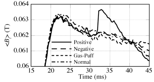
Fig.4 Time evolution of volume averaged toroidal magnetic field.
