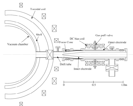
Fig.1 Schematic view of MCPG and a poloidal section of TPE-RX RFP
