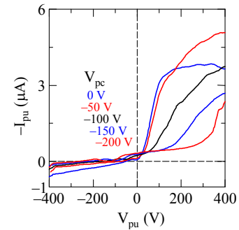
Fig. 4. Probe characteristics in the case of using the cylindrical porous cathode.
