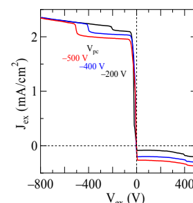
Fig. 2. Current-voltage characteristics of ion analyzer.
