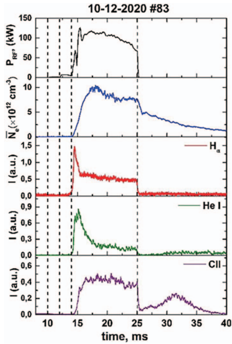
Fig. 3 Time evolutions of RF power; average plasma density; optical emission intensities of H_{\alpha} (656.2 nm), He I, (447.15 nm) and C II (426.7 nm). ( U_a = 8 kV, f = 4.9 MHz, B_0 = 0.35 T, K_{\varphi} = 0.32 , working gas 14% H_2 +86%He, p = 8.4 \times 10^{-3} Pa. The vertical lines show characteristic time moments of duty cycle of RF generator.)
