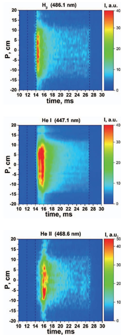
Fig. 4 Time evolution of H_{\beta} , He I and He II chord distribution. (12% H_2 +88%He, B_0 = 0.335 T, K_{\varphi} = 0.324 , f = 4.9 MHz, U_a = 7 kV, p = 9.974 \times 10^{-3} Pa. The vertical lines show time of duty cycle of RF generator.)
