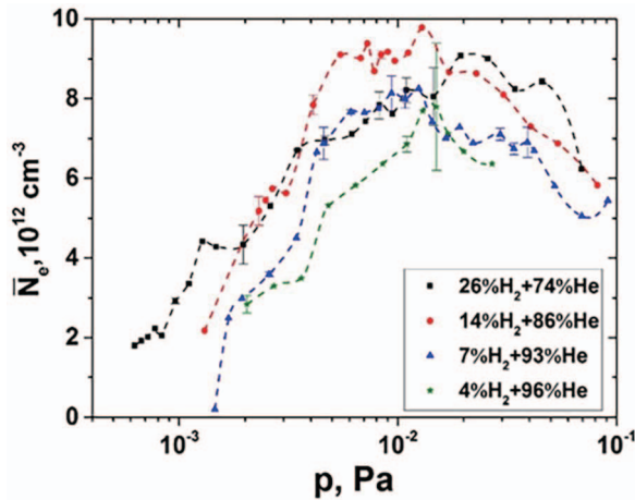
Fig. 5 Average plasma density as a function of the pressure ( U_a = 7 kV, f = 4.9 MHz). 26% H_2 +74%He ( B_0 = 0.34 T, K_q = 0.326 ), 14% H_2 +86%He ( B_0 = 0.35 T, K_q = 0.32 ), 7% H_2 +93%He ( B_0 = 0.35 T, K_q = 0.32 ), 4% H_2 +96%He ( B_0 = 0.344 T, K_q = 0.32 ).
