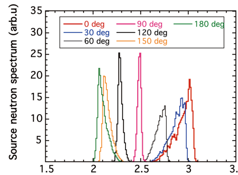
Fig. 4 Angular dependent neutron spectra at the target of the compact D-D neutron generator calculated by the PHITS code with double differential cross-section table for the \text{D(d, n)}^3\text{He} reaction. The emission angle is \theta in Fig. 1.
