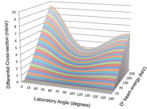
Fig. 3 Differential cross-section of the \text{D(d, n)}^3\text{He} reaction as a function of the incident deuteron energy. Here, 0 degree is the incident direction of the \text{D}^+ beam.
