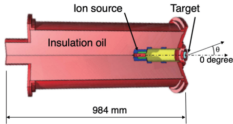
Fig. 1 Schematic view of the compact D-D neutron generator.
