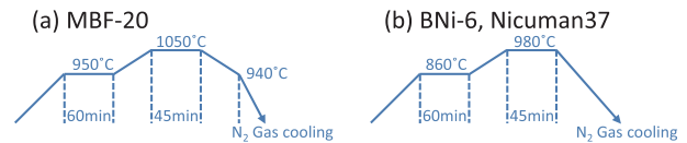
Fig. 2 Procedures of the heat treatment of (a) MBF-20 and (b) BNI-6 and Nicuman37 filler materials.
