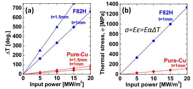
Fig. 1 (a) Temperature gradient as a function of an input power in different thickness of F82H ( 30 \text{ W/m}\cdot\text{K} ) and Pure-Cu ( 320 \text{ W/m}\cdot\text{K} ). (b) Induced internal thermal stress ( \sigma ) as a function of an input power in the 1 mm thickness of F82H and Pure-Cu. E : Young’s modulus [Pa], \alpha : Thermal expansion coefficient [ \text{K}^{-1} ].
