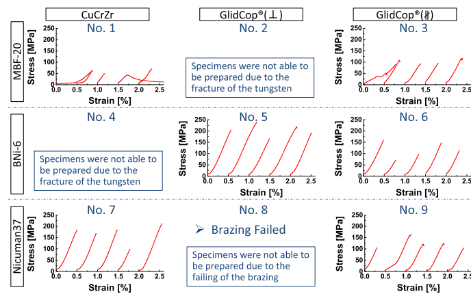
Fig. 3 Stress-strain curve of the three point bending test for the nine combination patterns of the copper alloys and the filler materials.
