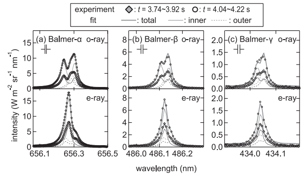
Fig. 4 Examples of the observed atomic spectra, (a) Balmer- \alpha , (b) -\beta , and (c) -\gamma lines, for the LOS4. The o-ray and e-ray components of the spectra are shown in the upper and lower parts of the figures, respectively. The spectra taken in t = 3.74\sim 3.92 s and 4.04\sim 4.22 s are shown by diamonds and circles, respectively. The instrumental width for each wavelength region is shown by the interval of the vertical lines. The fitted results are shown by bold curves. The estimated spectra of the emissions from the inboard and outboard emission locations are shown by thin solid and dotted curves, respectively.
