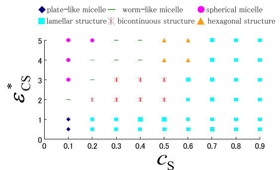
Fig. 1 Hydrophilic interaction parameter vs. bolaamphiphilic concentration phase diagram of bolaamphiphilic molecules.
