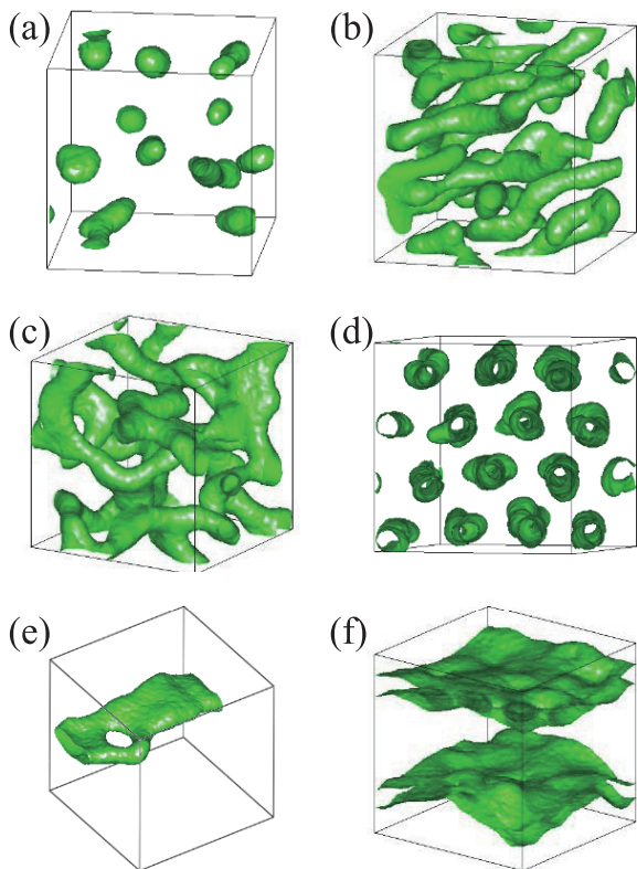
Fig. 2 Snapshots of various self-assembled structures formed by bolaamphiphilic molecules. (a) Spherical micelles, (b) worm-like micelles, (c) bicontinuous structure, (d) hexagonal structure, (e) plate-like micelles, and (f) lamellar structure.
