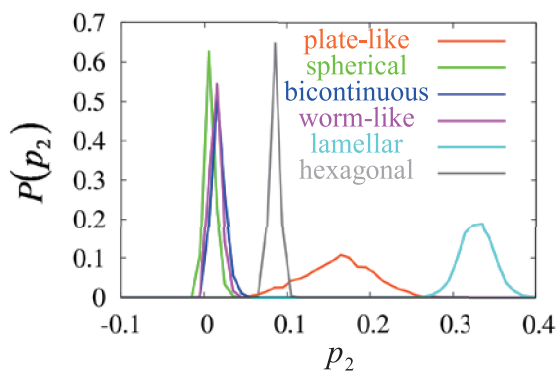
Fig. 3 Distribution function of the global orientational order parameter for the end bonds of the bolaamphiphilic molecules P(p_2) for six kinds of self-assembled structures.
