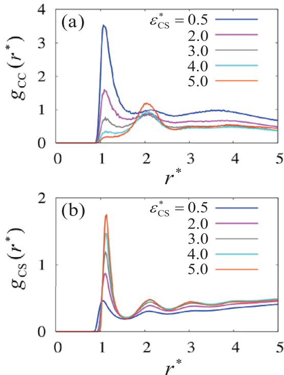
Fig. 4 The radial distribution function (a) between hydrophilic particles C, g_{CC}(r^*) , and (b) between hydrophilic particles C and solvent particles S, g_{CS}(r^*) , in the case of c_S = 0.1 .
