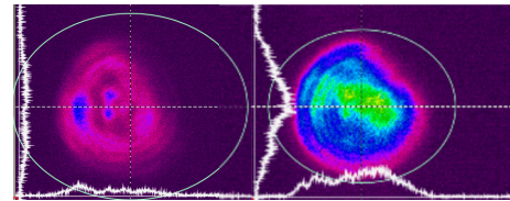
Fig. 3 Beam profile for only the first pass (left) compared with that for all multiple-passes (right).
