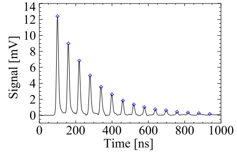
Fig. 2 Signal at the photodiode detector. Blue diamonds mark observed peaks for each round trip.
