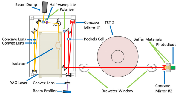
Fig. 1 Schematic of the optical system for multi-pass Thomson scattering (TS) and the measurement setup in TST-2. A laser pulse can be confined between concave mirror #1 and concave mirror #2 (red lines).
