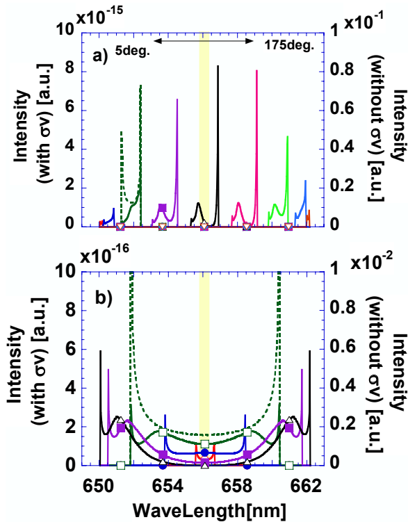
Fig. 3 Expected FIDA spectra of (a) tangential- and (b) perp.-LOSs for mono-energetic particles of 80 keV. The particles of having pitch angles of 5( \circ ), 22.5( \bullet ), 45( \square ), 67.5( \blacksquare ), 90( \triangle ), 112.5( \blacktriangle ), 135( \diamond ), 157.5( \blacklozenge ), and 175 deg.( \nabla ) are shown. For the particle with a 45 degree pitch angle, the spectra without considering the effect of emission reactivity are shown by dashed curves. Yellow shaded area shows the expected region where cold D_\alpha spectra can be observed.
