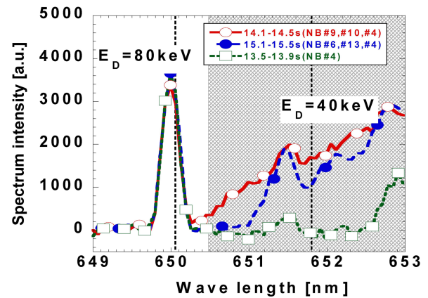
Fig. 4 Typical FIDA spectra measured on JT60U (at R = 3.4 m) for tangential-NB plus probe-NB injection( \circ ), perp.-NB plus probe-NB injection( \bullet ), and probe-NB only injection( \square ) are shown.
