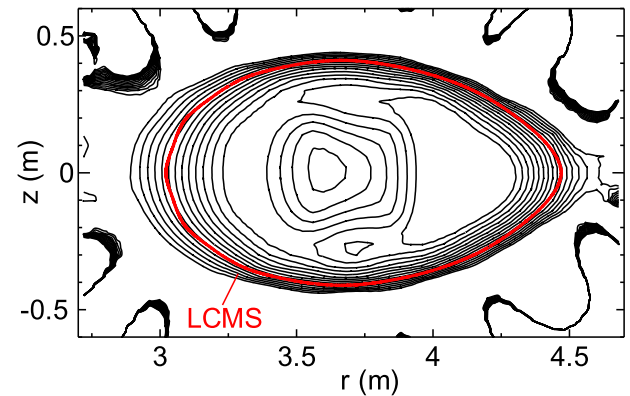
Fig. 13 Contours of quasi magnetic surface.
