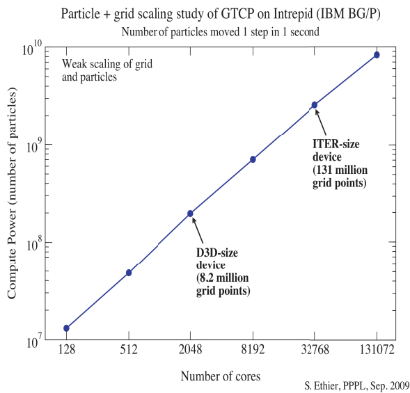
Fig. 1 Speedups of the GTC-P code on the quad-core IBM Blue-Gene-P (results courtesy of S. Ethier)
