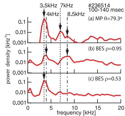
Fig. 3 Power density spectra of (a) the magnetic fluctuation, (b) the density fluctuation at \rho = 0.95 , and (c) the density fluctuation at \rho = 0.53 .
