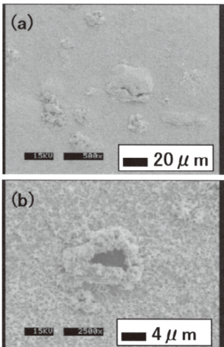
Fig. 4 Surface modification of the blister-rich surface of W1 due to He plasma exposure at 2,000 K for 1 hour. (a) Some blisters have collapsed. (b) A clearly collapsed blister and porous structure with a diameter of 200–300 nm, which is usually formed due to He plasma exposure at high temperatures, are observed on the surface.
