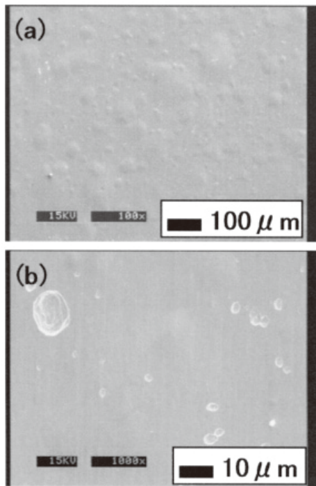
Fig. 2 Surface modification of sample W1 after deuterium plasma exposure at 500 K for 3 hours. (a) Many blisters with sizes up to \sim 200 \mu\text{m} are observed. (b) Some blisters of less than \sim 10 \mu\text{m} in size are exfoliated. No blister exfoliation was observed for large blisters, that is, those larger than \sim 10 \mu\text{m} .
