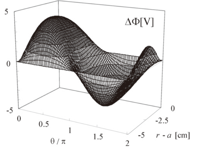
Fig. 3 A two-dimensional potential perturbation profile with small and homogeneous E_r .
