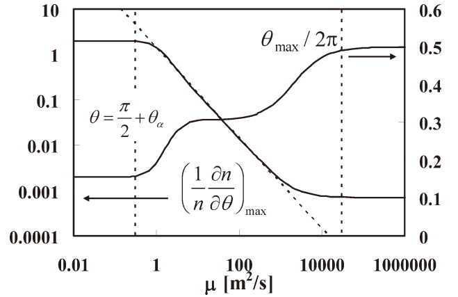
Fig. 4 Relationship between shear viscosity \mu and the poloidal shock structure. The steepness and the position of the shock are important for describing the structure.
