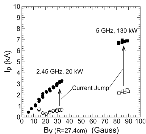
Fig. 4 Plasma current versus external vertical field strength.
