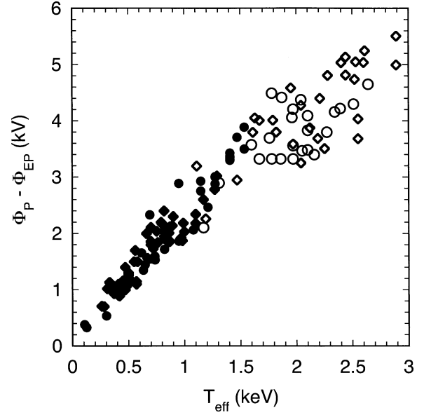
Fig. 8 Scaling law between \Phi_P - \Phi_{EP} and T_{\text{eff}} . The closed circles indicate data obtained with P_{\text{plug}} below the nominal power. The open symbols stand for the high power heating. In addition, open circles denote \Delta\Phi from hot ion mode plasmas and open diamonds represent those from high potential mode plasmas.
