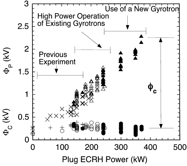
Fig. 4 \Phi_P and \Phi_C are plotted as functions of P_{\text{plug}} . Data are taken from the three stages of the GAMMA 10 experiment: data from the previous experiment (denoted with crosses), data from the first step experiment (open triangles), and data from the second step experiment with the new high power gyrotron (closed triangles).
