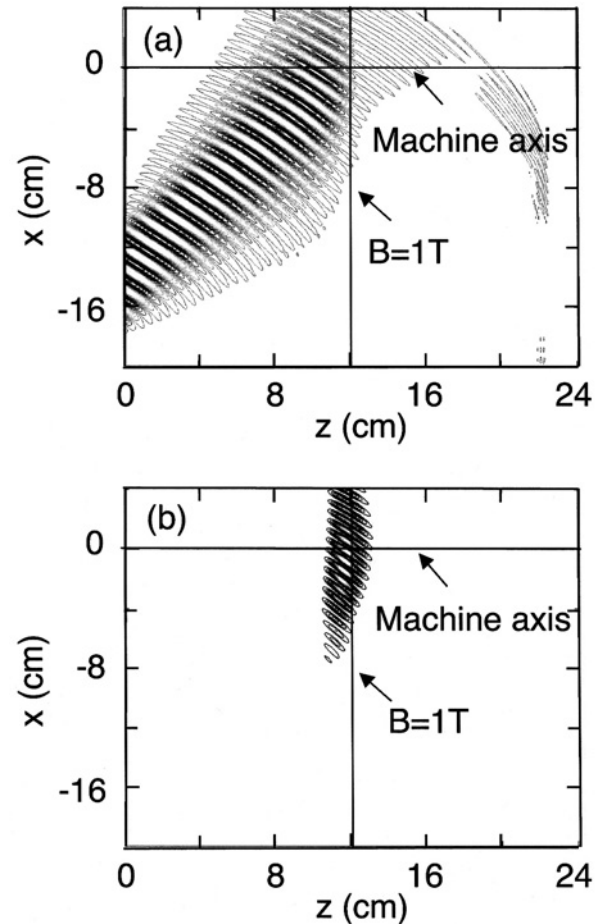
Fig. 10 Propagation of the heating wave calculated by using a full Maxwellian code is shown. The heating wave is launched from the high field side and propagates up right with the same angle to the machine axis as that in experiment. It is excited in linear polarization along the y direction. (a) The amplitude distribution of the wave electric field. (b) Wave absorption profile. The two profiles plotted in Figs. (a) and (b) stand for snap shots at a certain instant.
