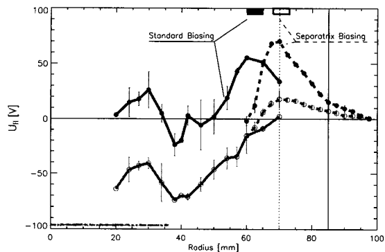
Fig. 6 Comparison of the radial profile of the floating potential with and without biasing ( U_b = +100 V), plotted for two positions of the biasing electrode: r_{bias} = 60 mm – “standard” biasing scheme (solid lines), measured by a single floating probe on a shot-to-shot basis; r_{bias} = 68 mm – “separatrix” biasing (dashed lines), measured by a rake probe.
