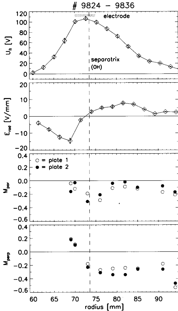
Fig. 7 Radial profiles at separatrix biasing ( U_b = +150 V). Top panels: floating potential and radial electric field ( E_r = -\nabla U_{fl} , neglecting \nabla T_e with biasing). Bottom panels: parallel and perpendicular Mach numbers deduced from both plates (plate 1. - \circ , plate 2. - \bullet ). The dashed vertical line denotes the position of the separatrix in the non-polarized discharges.
